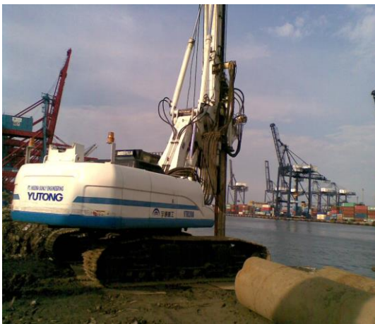
YUTONG YTR 200, in TANJUNG PRIOK.
